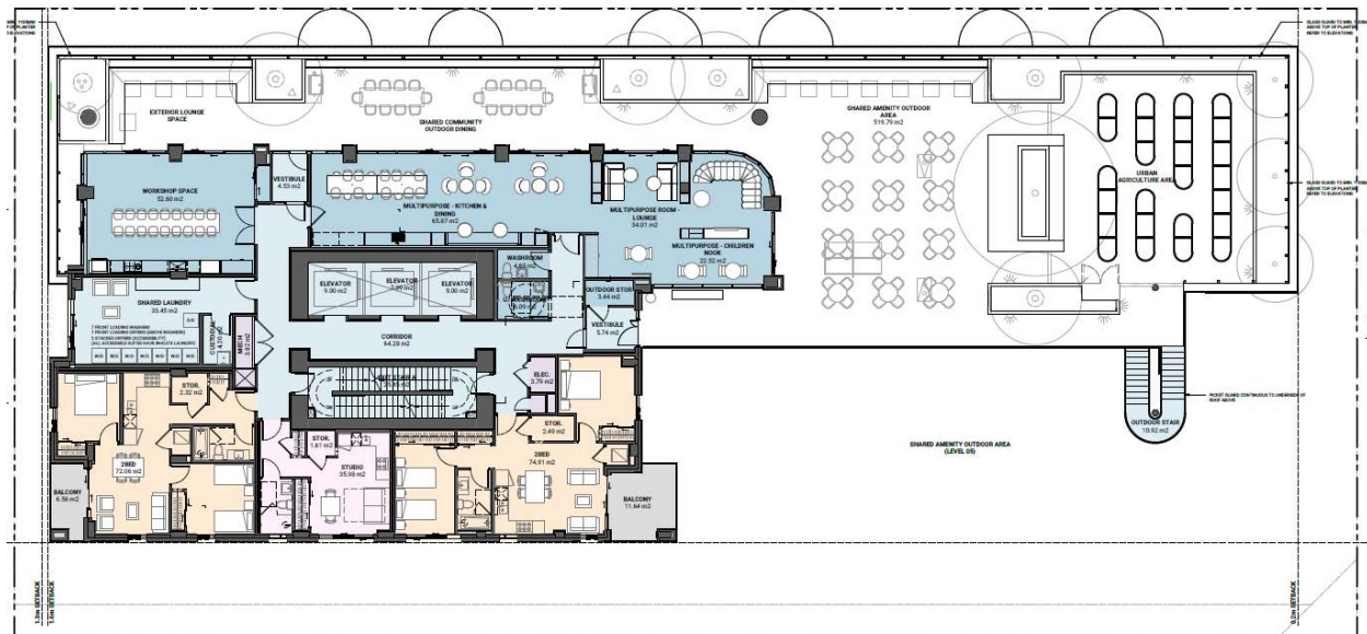
Level 12 Floor Plan
