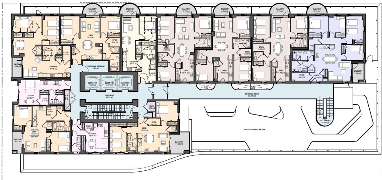
Level 6 Floor Plan
