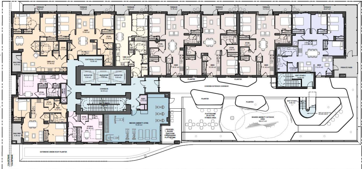
Level 5 Floor Plan
