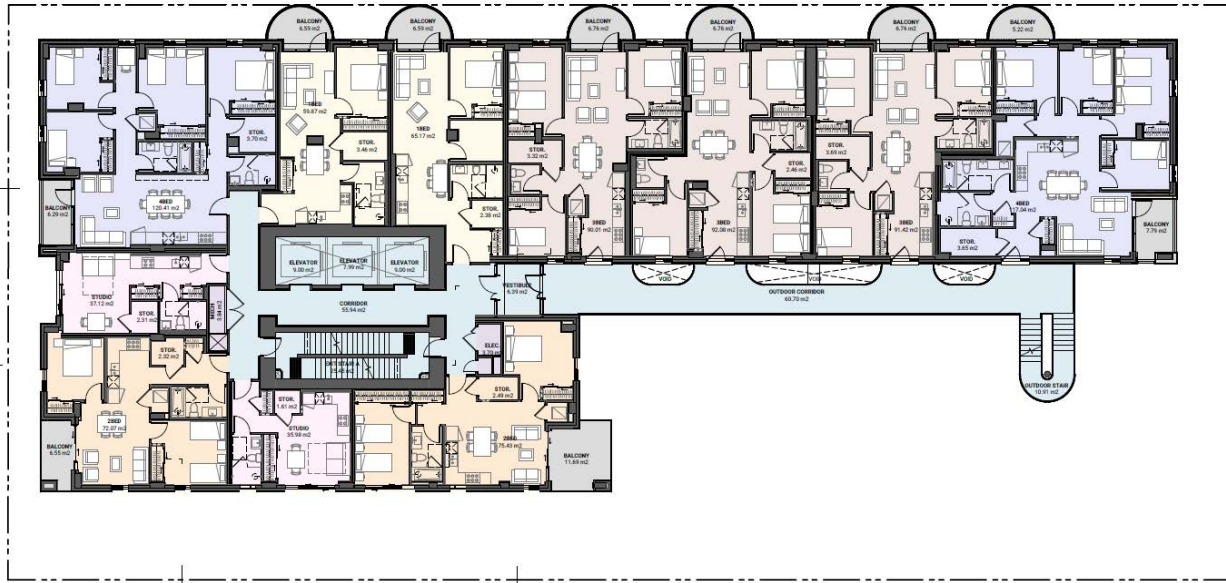
Levels 9 to 11 Floor Plan
