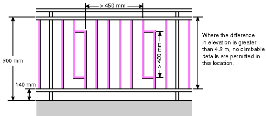
Figure A-9.8.8.6.(1)-A Example of minimum horizontal and vertical clearances between protrusions in guards
