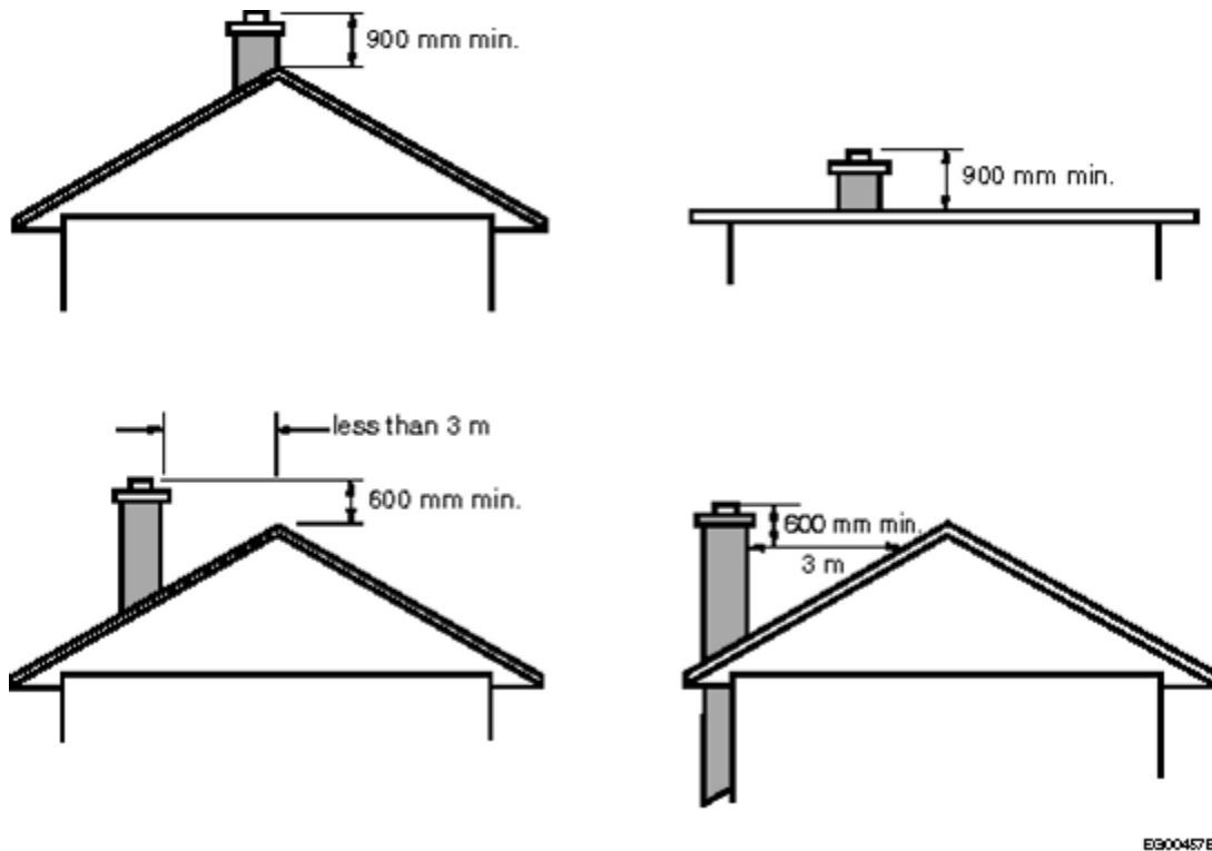
Figure A-9.21.4.4.(1)
