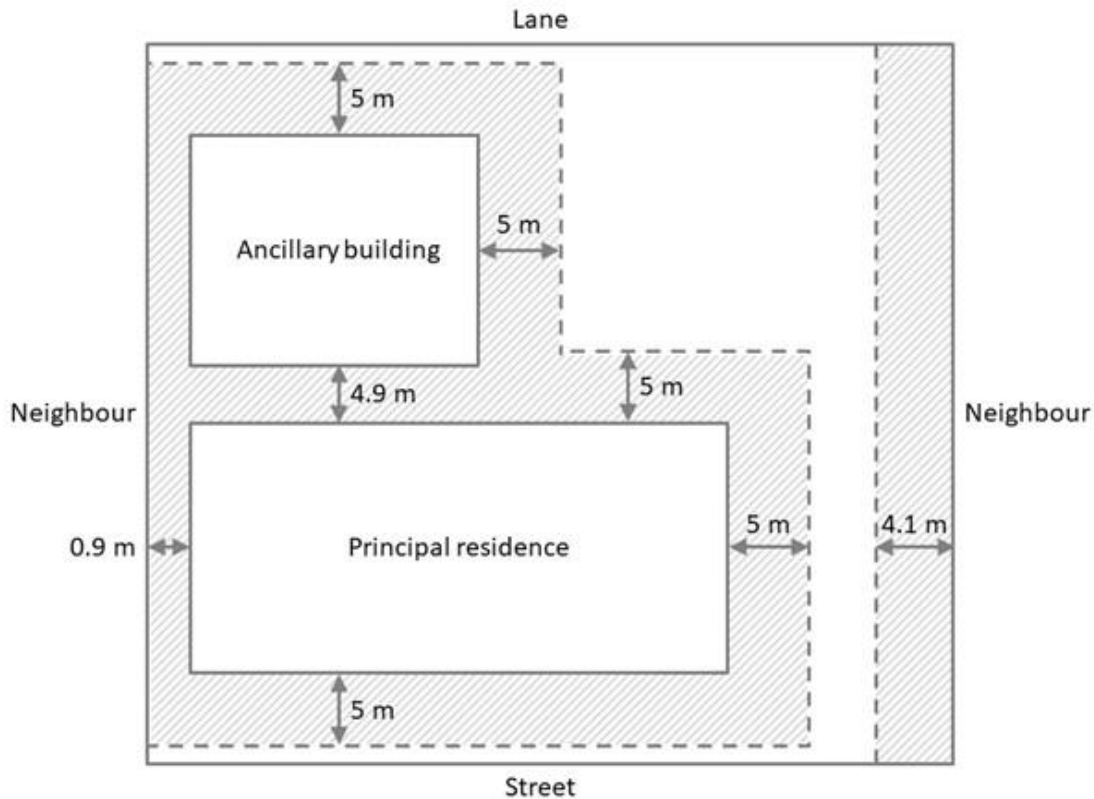
Figure A-9.14.5.3.(2) Minimum setbacks for on-site infiltration systems from buildings and neighbouring properties. Not to scale.
