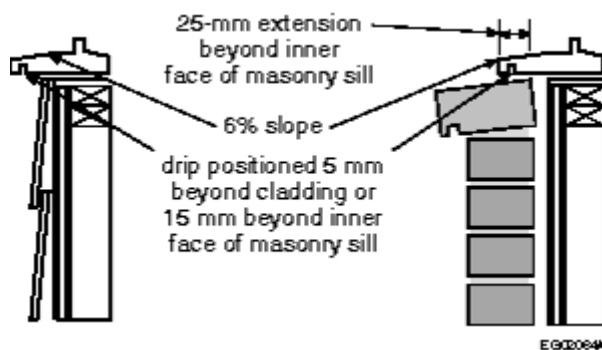
Figure A-9.27.3.8.(5)
