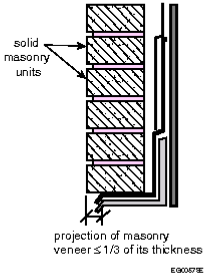
Figure A-9.20.8.5.(1)
