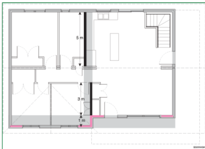
Figure A-9.23.13.6.(5)-B
