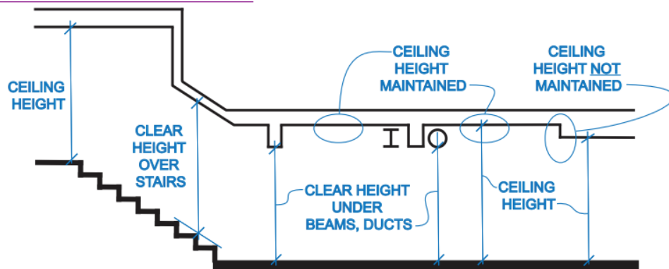
Figure A-9.5.3.1. Ceiling Heights and Clear Heights
