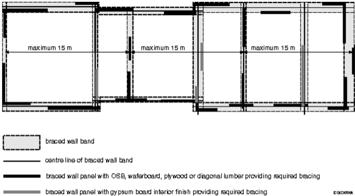
Figure A-9.23.13.6.(3)
