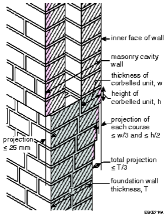
Figure A-9.20.12.2.(2)
