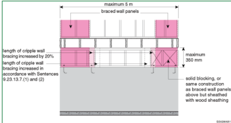
Figure A-9.23.13.8.(3)
