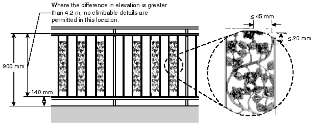
Figure A-9.8.8.6.(1)-C Example of a guard with spaces that are not more than 45 mm wide and 20 mm high
