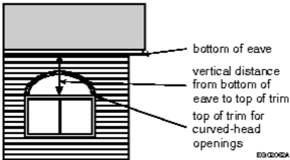
Figure A-9.27.3.8.(3)
