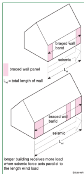
Figure A-9.23.13.7.(4)-A
