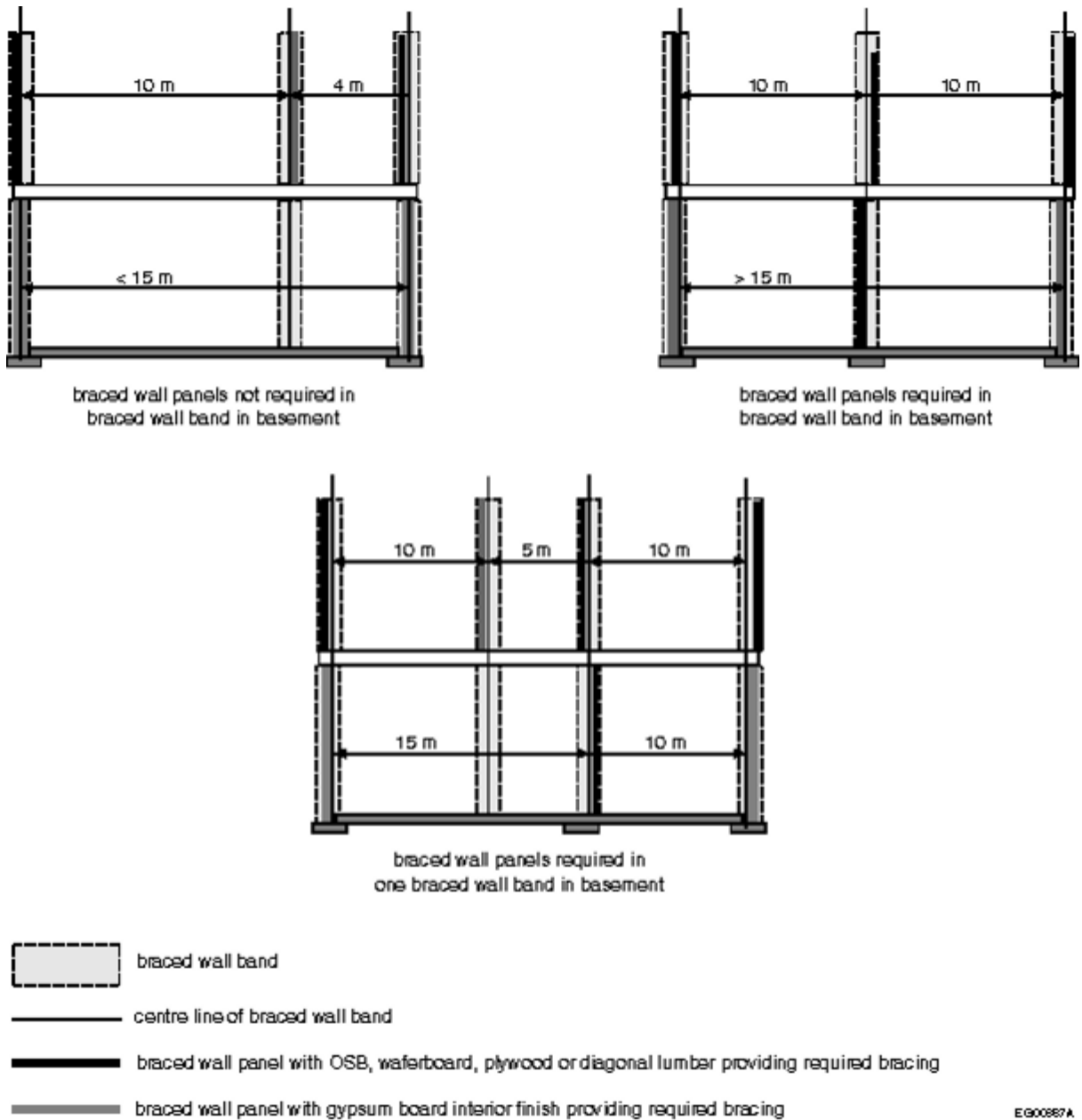
Figure A-9.23.13.5.(2)
