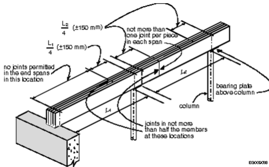
Figure A-9.23.8.3.
