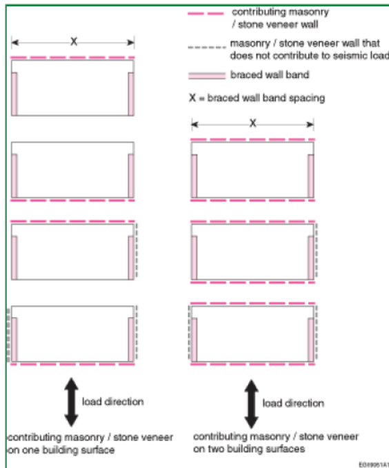
Figure A-9.23.13.7.(4)-D
