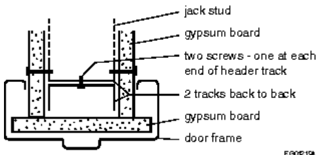
Figure A-9.24.3.2.(3)
