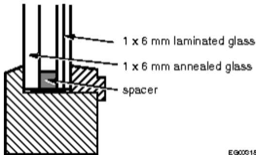
Figure A-9.7.5.2.(1) Combined laminated/annealed glazing
