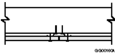
Figure A-9.10.3.1.-A Single layer butt joint details
