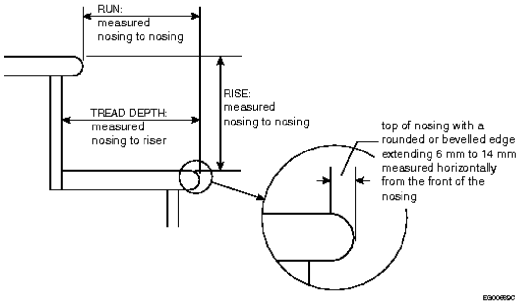
Figure A-9.8.4.-B Step dimensions and their measurement
