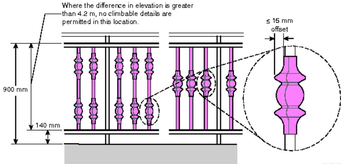
Figure A-9.8.8.6.(1)-B Examples of maximum horizontal offset of protrusions in guards
