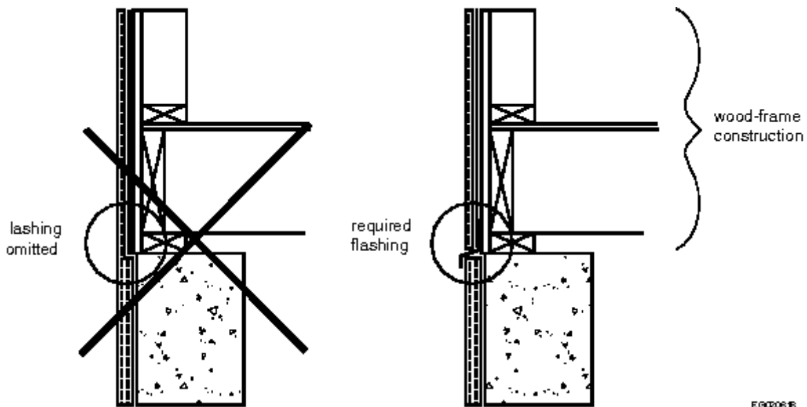
Figure A-9.27.3.8.(1)
