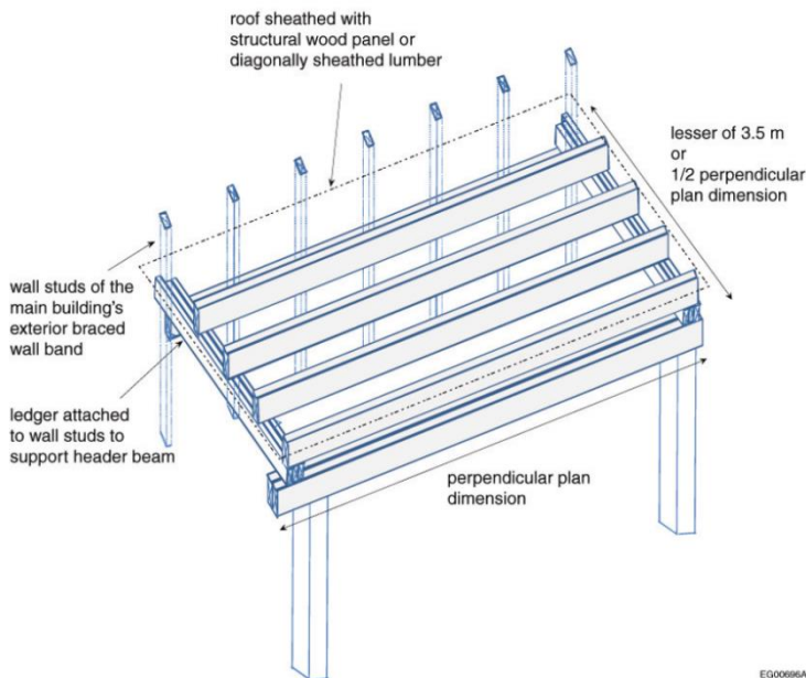
Figure A-9.23.13.10.(2)-B
