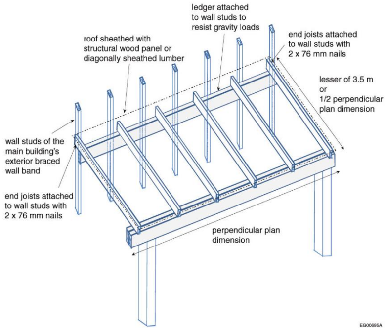
Figure A-9.23.13.10.(2)-A
