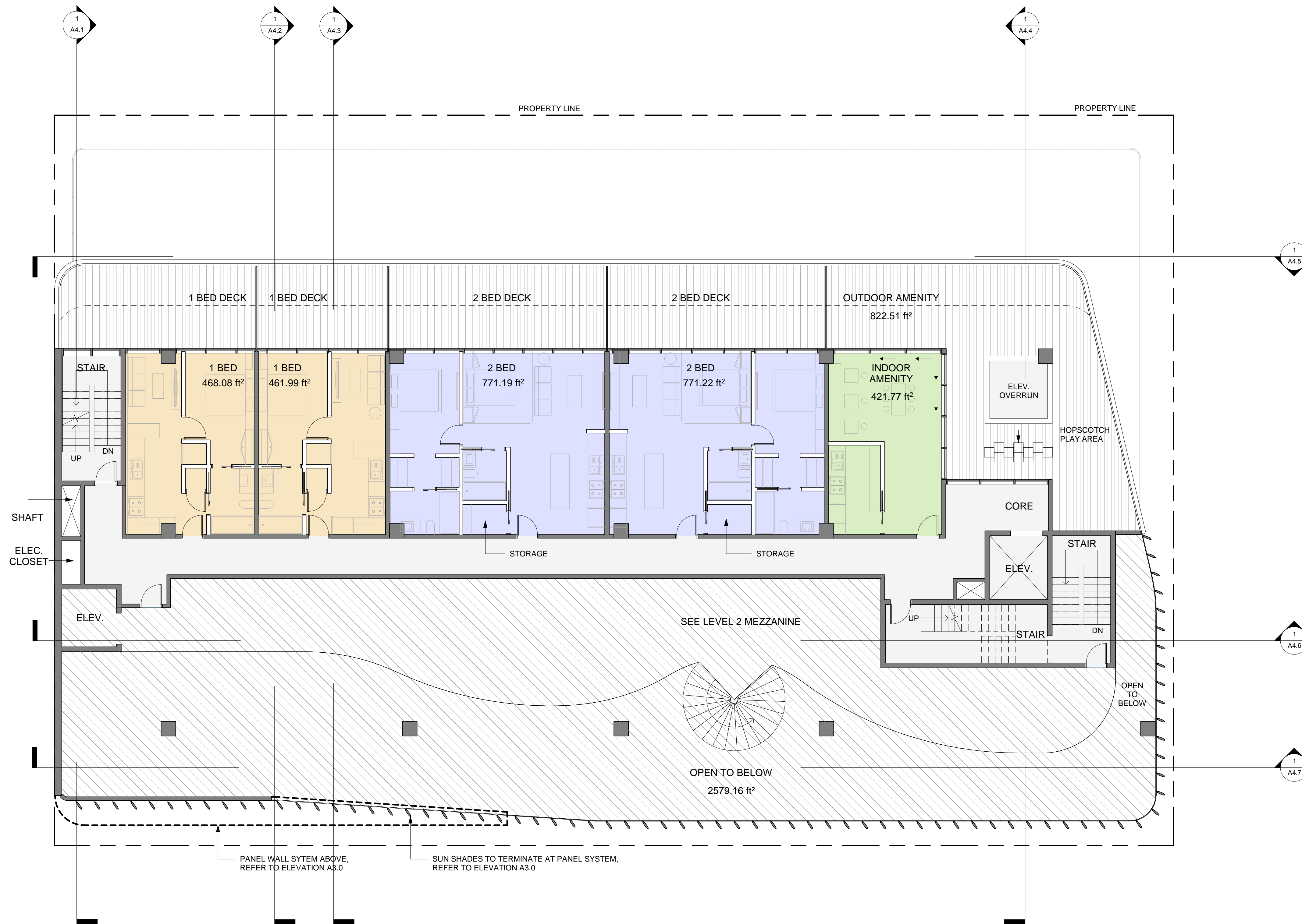
1 LEVEL 3 - RESIDENTIAL 1/8" = 1'-0"
