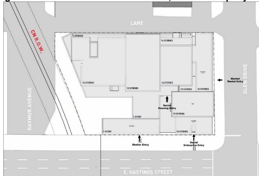
Figure 8: 5m Setback from CN Rail ROW, on West Property Line
