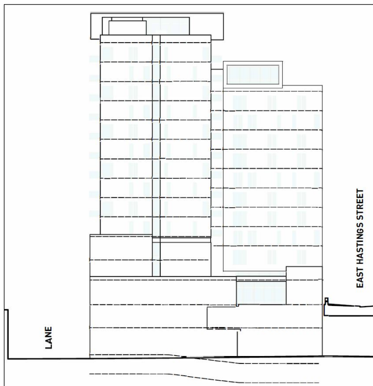
West Elevation
