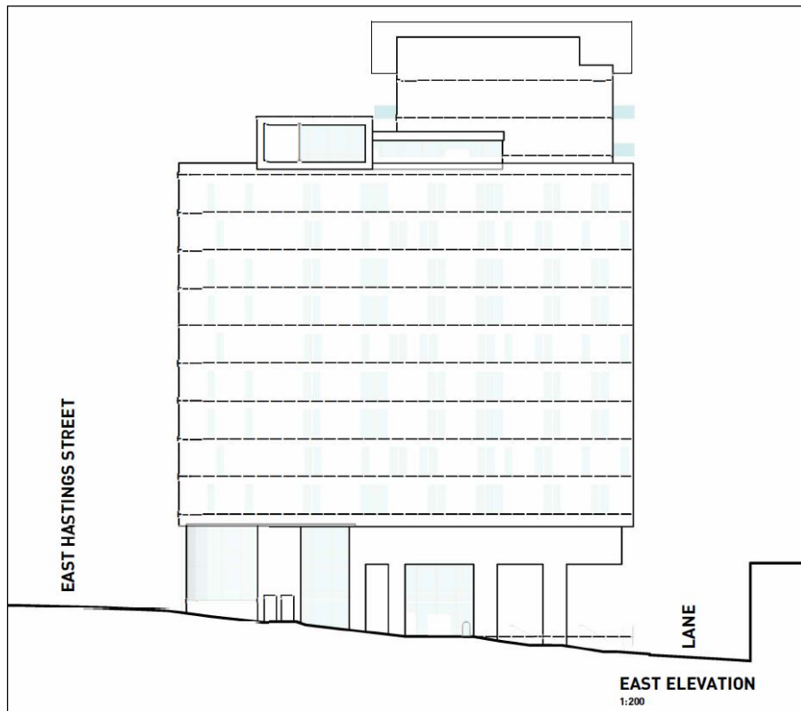
East Elevation
