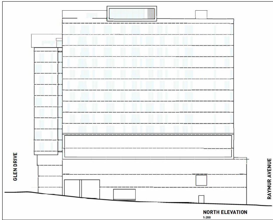
North Elevation
