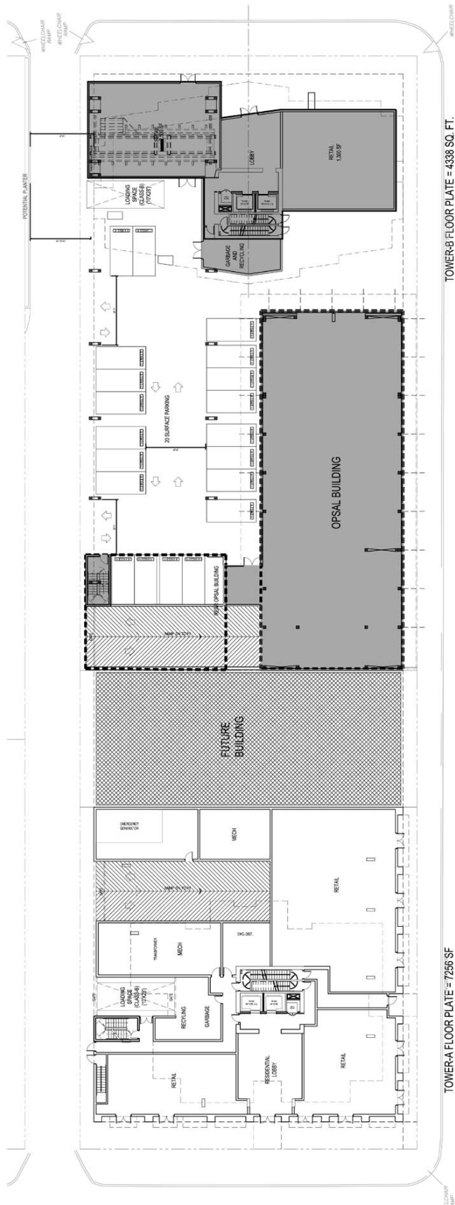
1 FIRST FLOOR PLAN SCALE 1/16"=1'-0"
