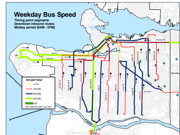
Figure 11 Midday Bus Speeds Inbound to Downtown
