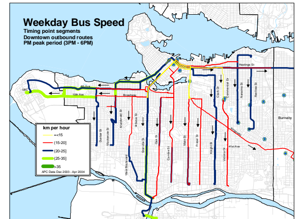
Figure 12 PM Peak Bus Speeds Outbound from Downtown
