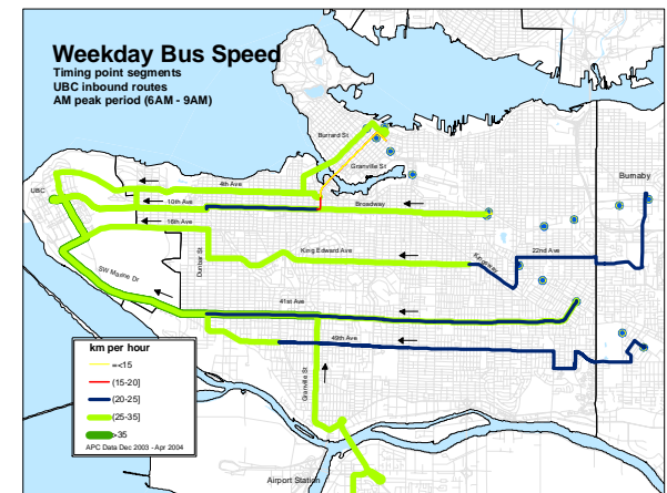
Figure 13 AM Peak Bus Speeds Inbound to UBC
