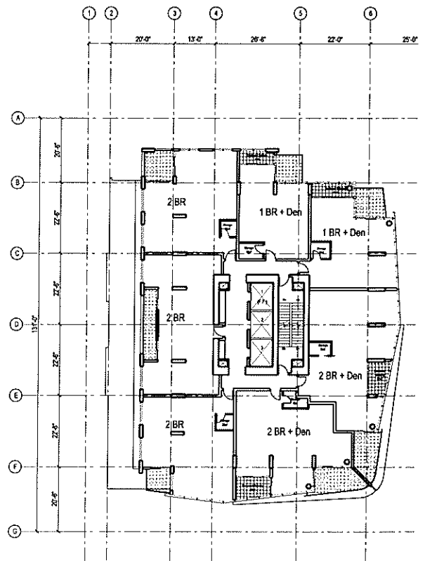
Level 29 to 36 - Residential
