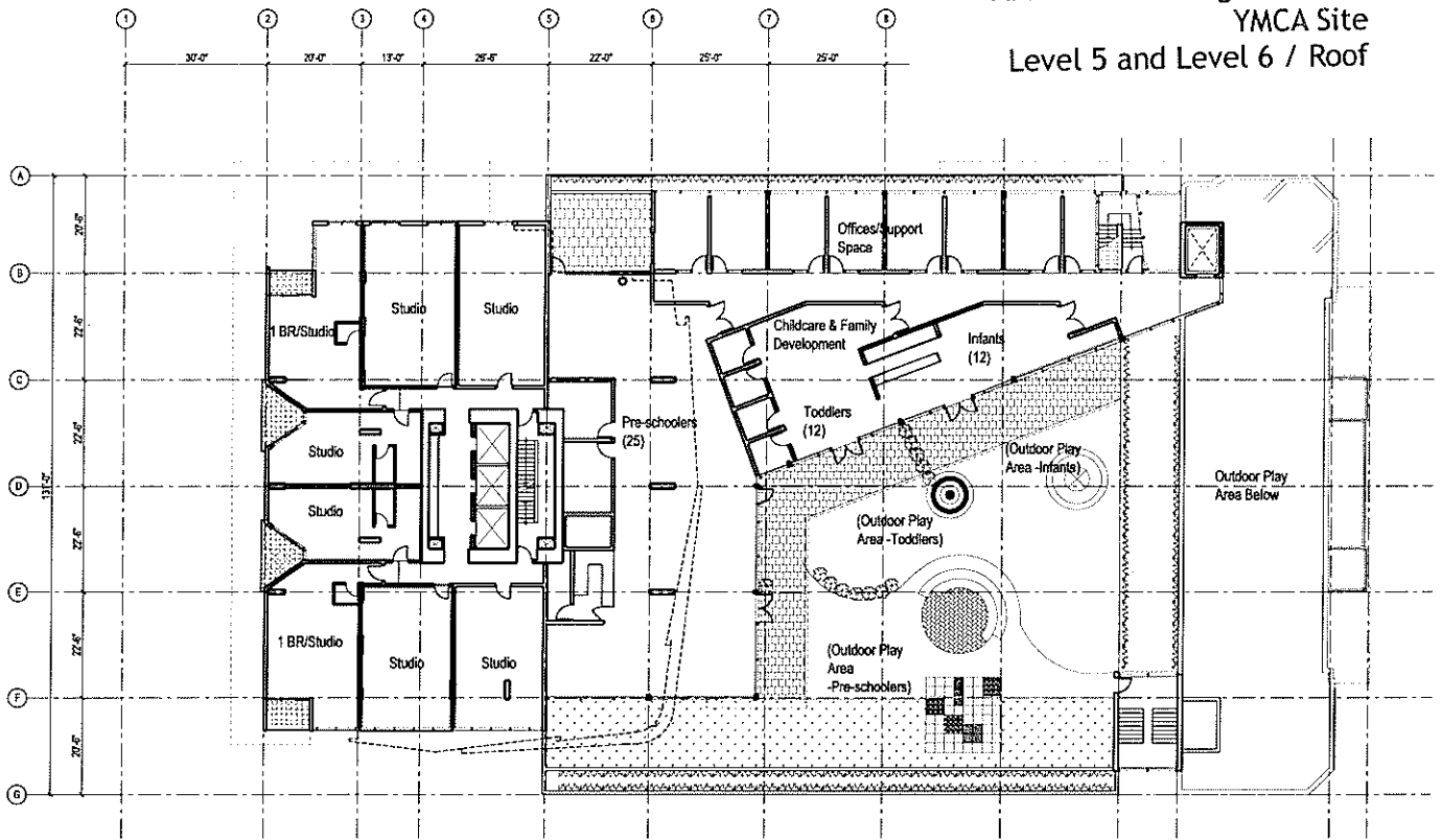
Level 6 / Childcare & Family Development El. 65.0
