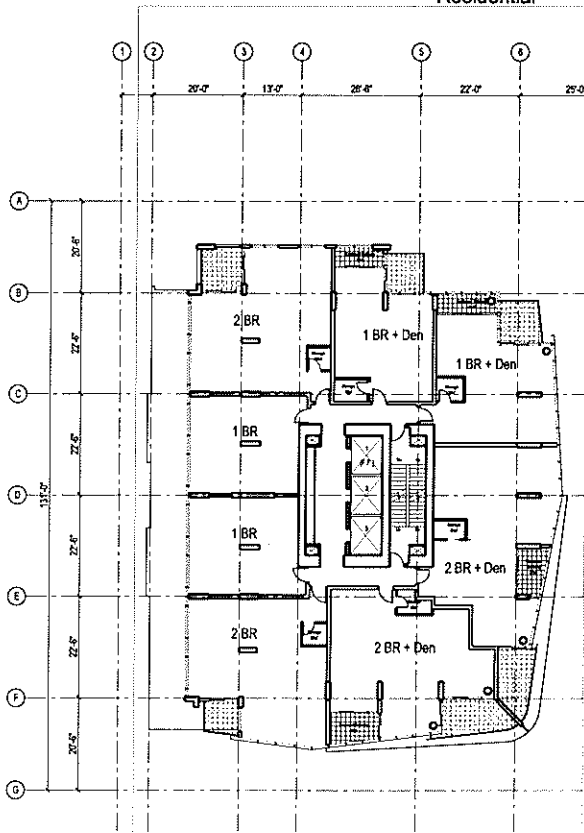
Level 14 to 28 - Residential
