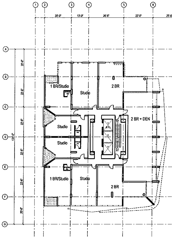
Level 8 -Residential
