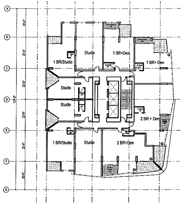
Level 9 to 13 - Residential
