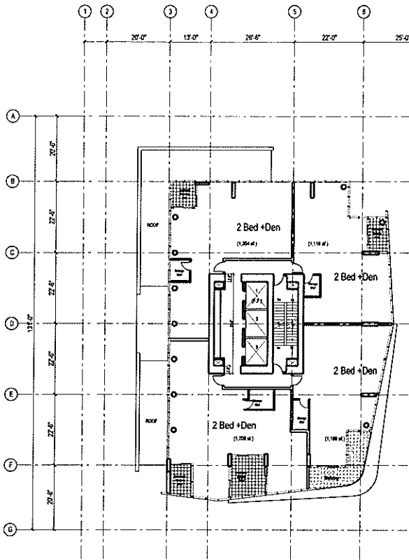
Level 37 to 40 - Residential
