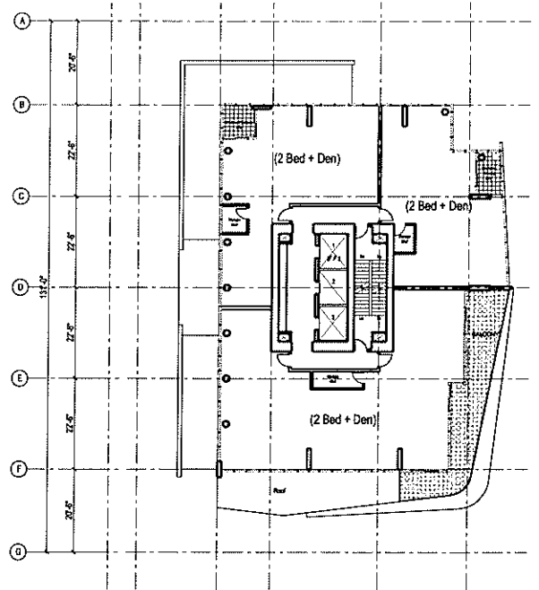
Level 42 - Residential
