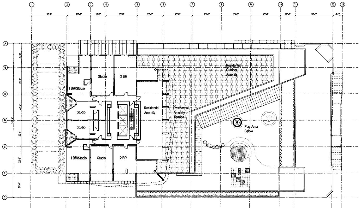
Level 7 - Residential / YMCA Roof
