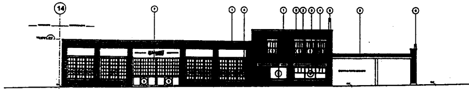
NORTH ELEVATION
