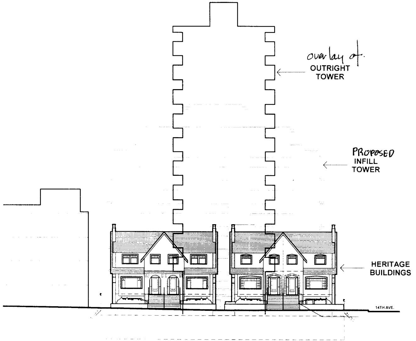
SOUTH ELEVATION - SHOWING OUTRIGHT TOWER
