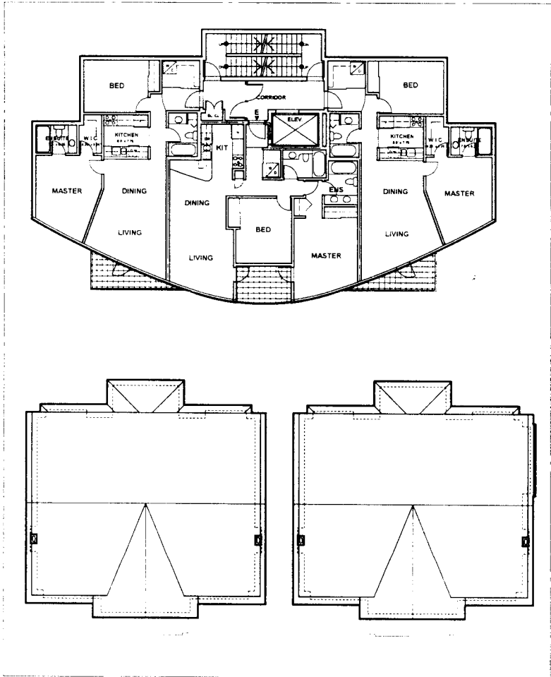
4TH TO 7TH FLOOR PLANS
