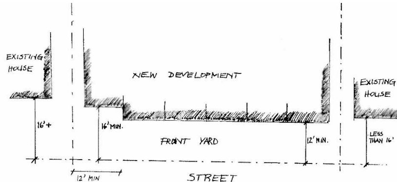
Figure 13: Front yard setbacks depend on the setback of adjacent buildings
