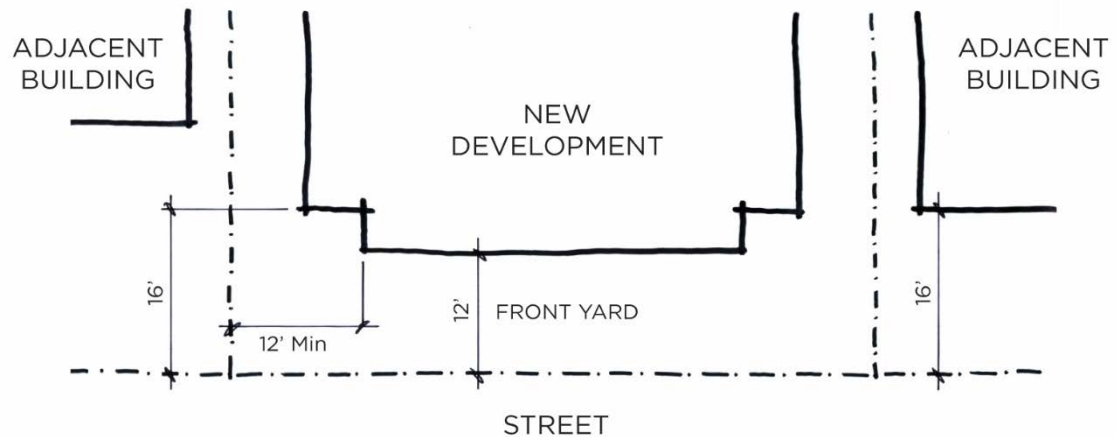
Figure 10: Front yard setbacks depend on the setback of adjacent buildings in RM-9, RM-9N and RM-9BN
