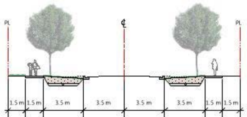
LOCAL STREET - INFILTRATION BULGES Scale 1:200
